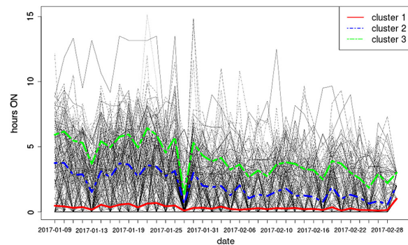
Fig. 9. Cluster evolutions.
