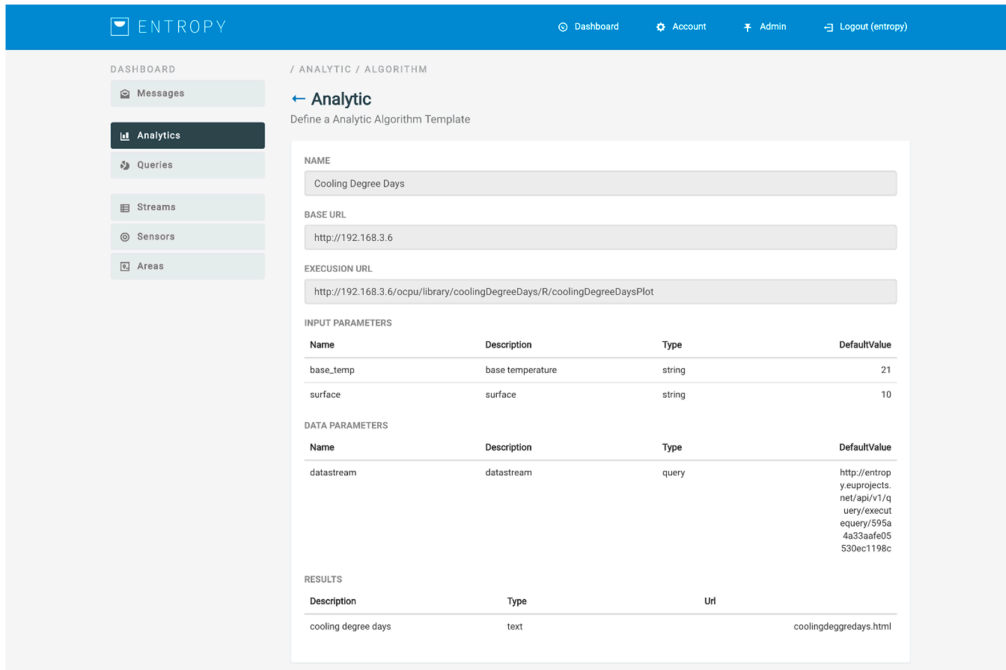
Figure 9. Indicative algorithm analysis template.
