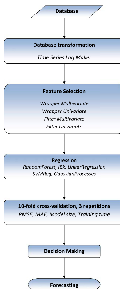
Fig. 2. Methodology for feature selection for energy time series forecasting.
