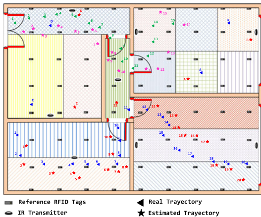
Fig. 4. Tracking processes with a reference tag distribution of 1 \text{ m} \times 1 \text{ m} .
