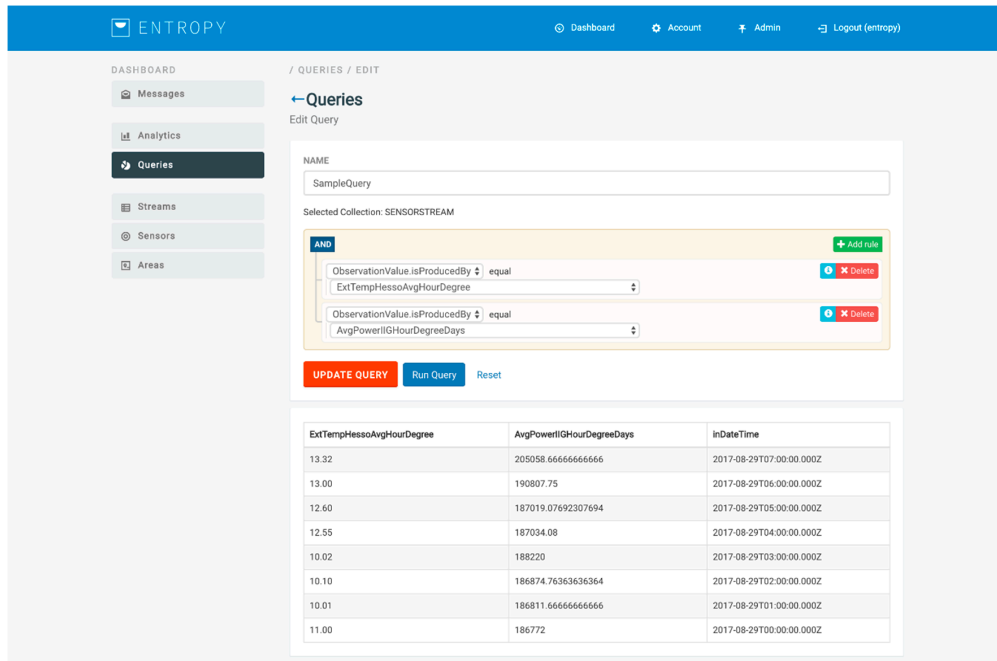
Figure 10. Indicative query design through the query builder.
