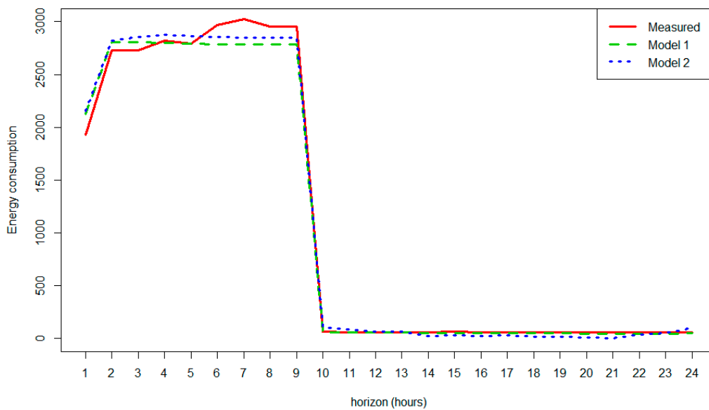
Figure 11. Energy consumption-real measures vs prediction (Model 1/Model 2).
